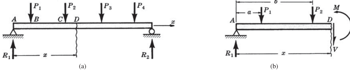
Fig. 6-6 Several forces acting on a simple beam.
