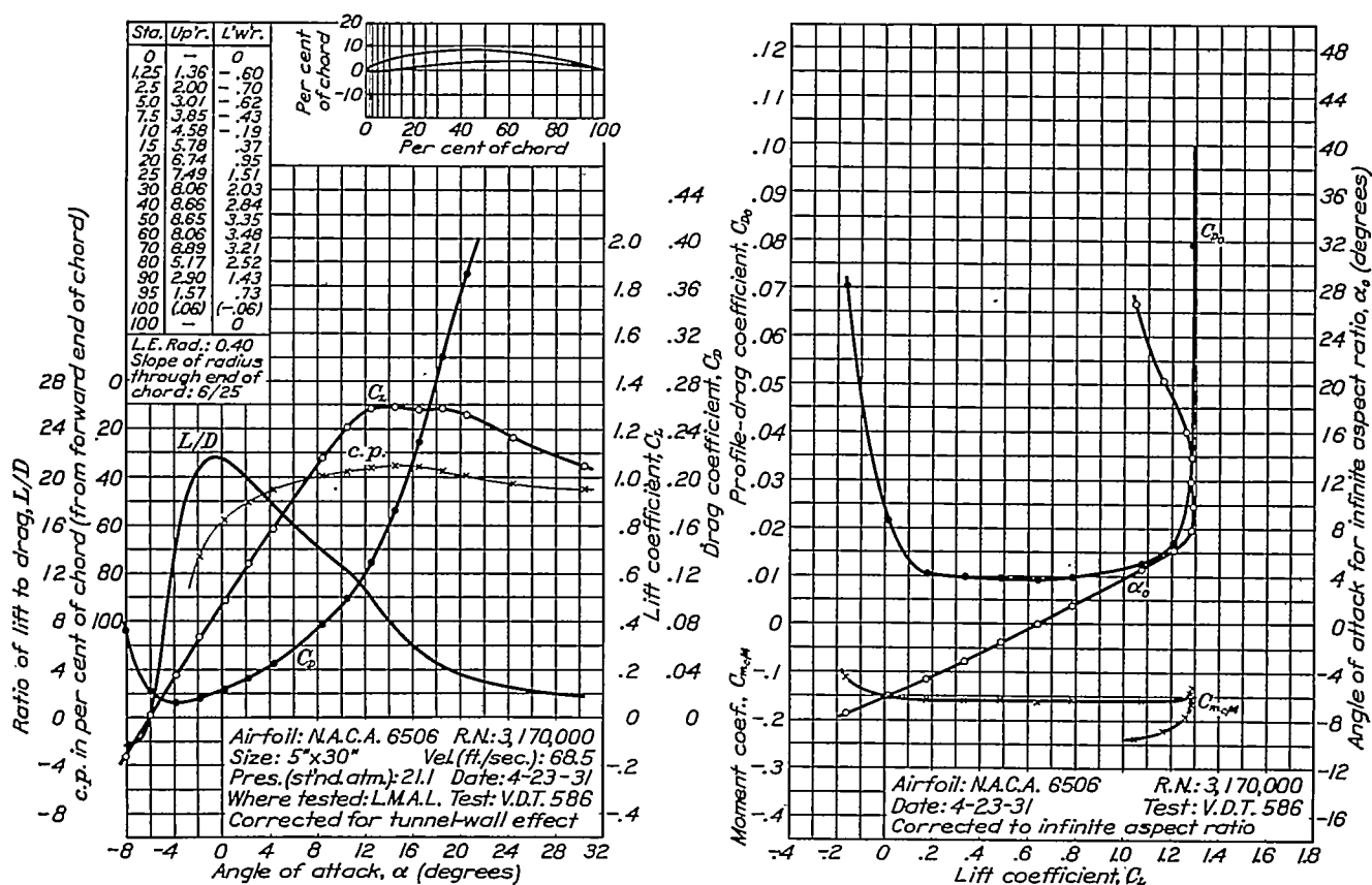
FIGURE 64.—N.A.C.A. 6506 airfoil.
