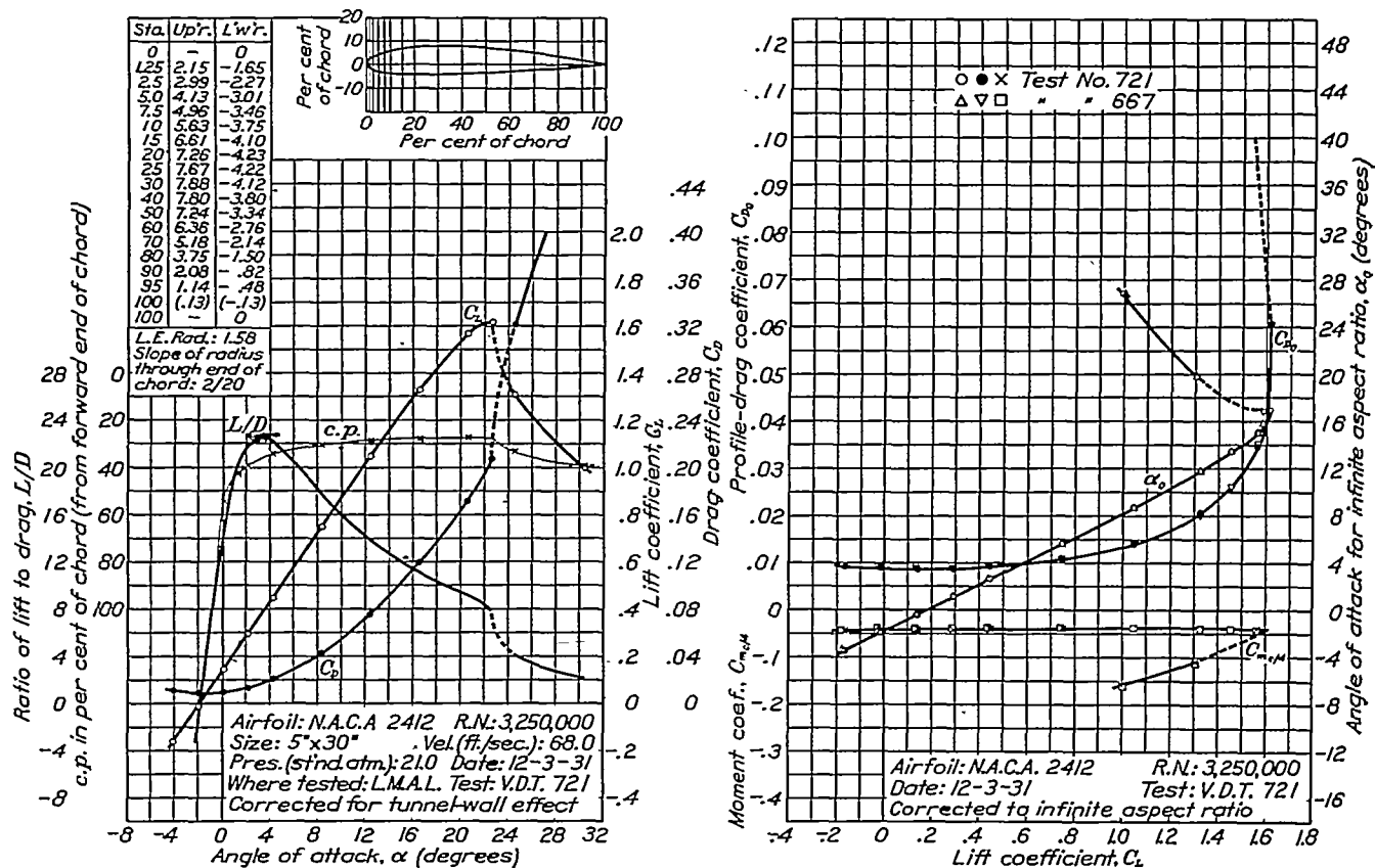
FIGURE 18.—N.A.C.A. 2412 airfoil.
