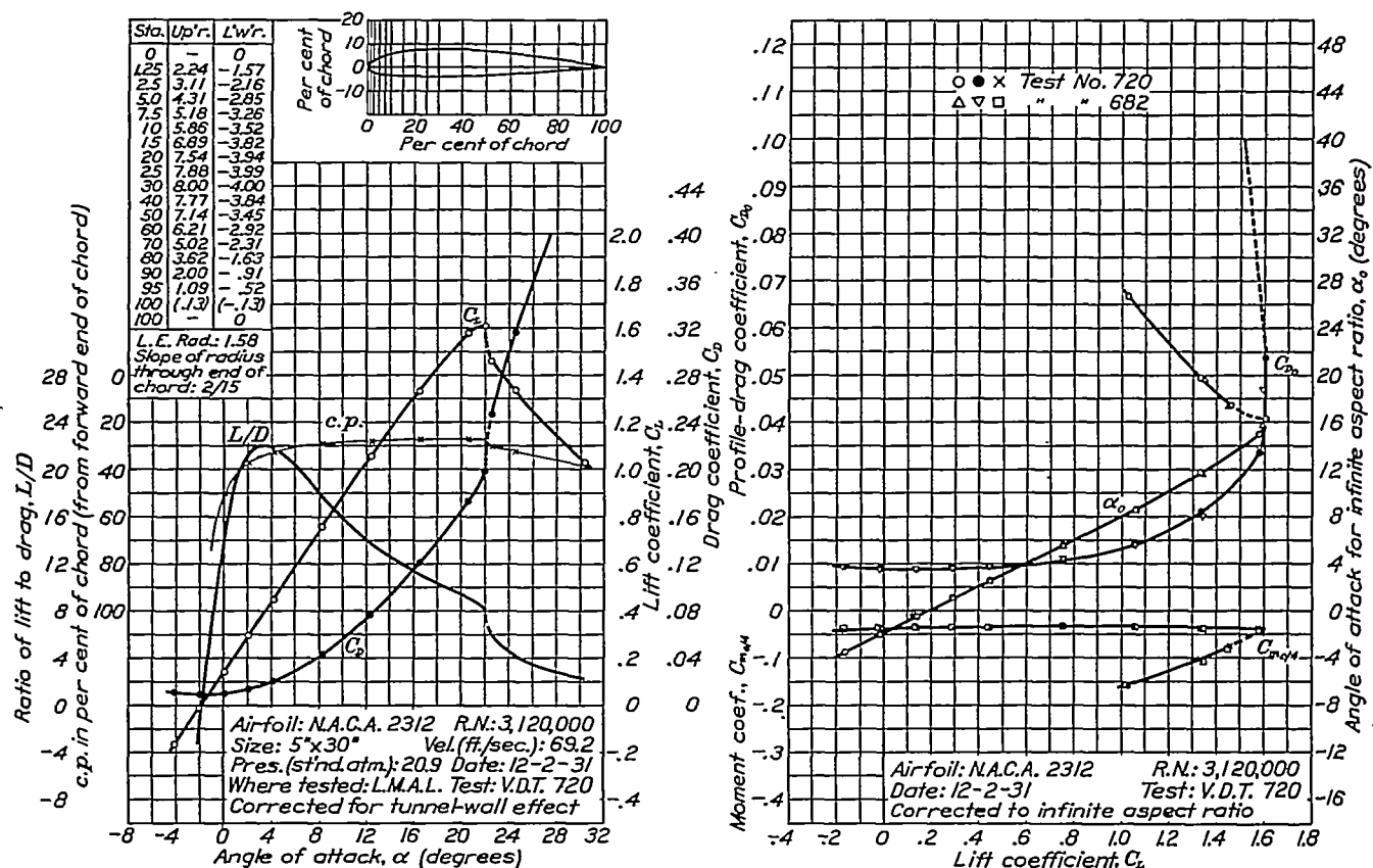
FIGURE 14.—N.A.C.A. 2312 airfoil.
