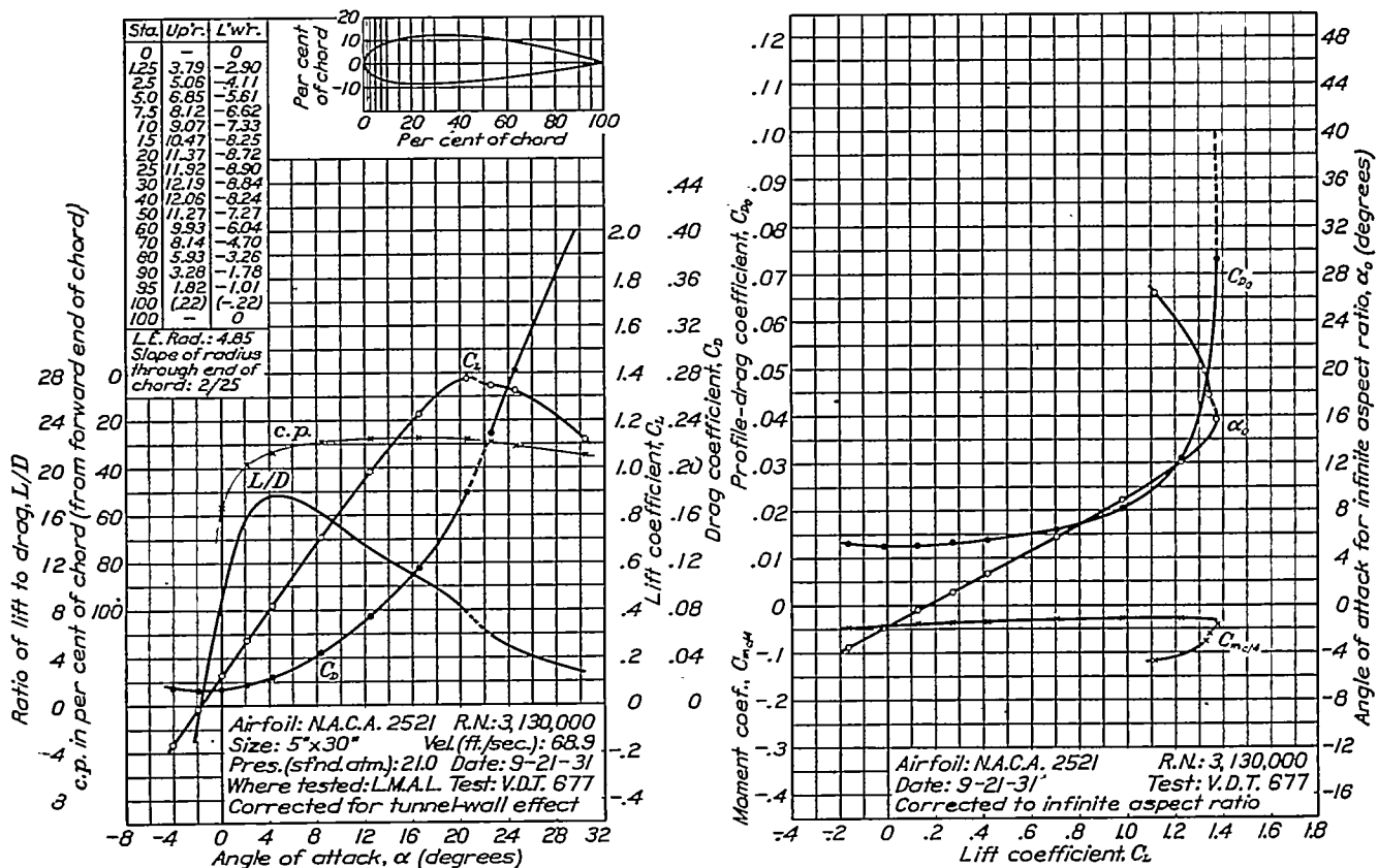
FIGURE 27.—N.A.C.A. 2521 airfoil.
