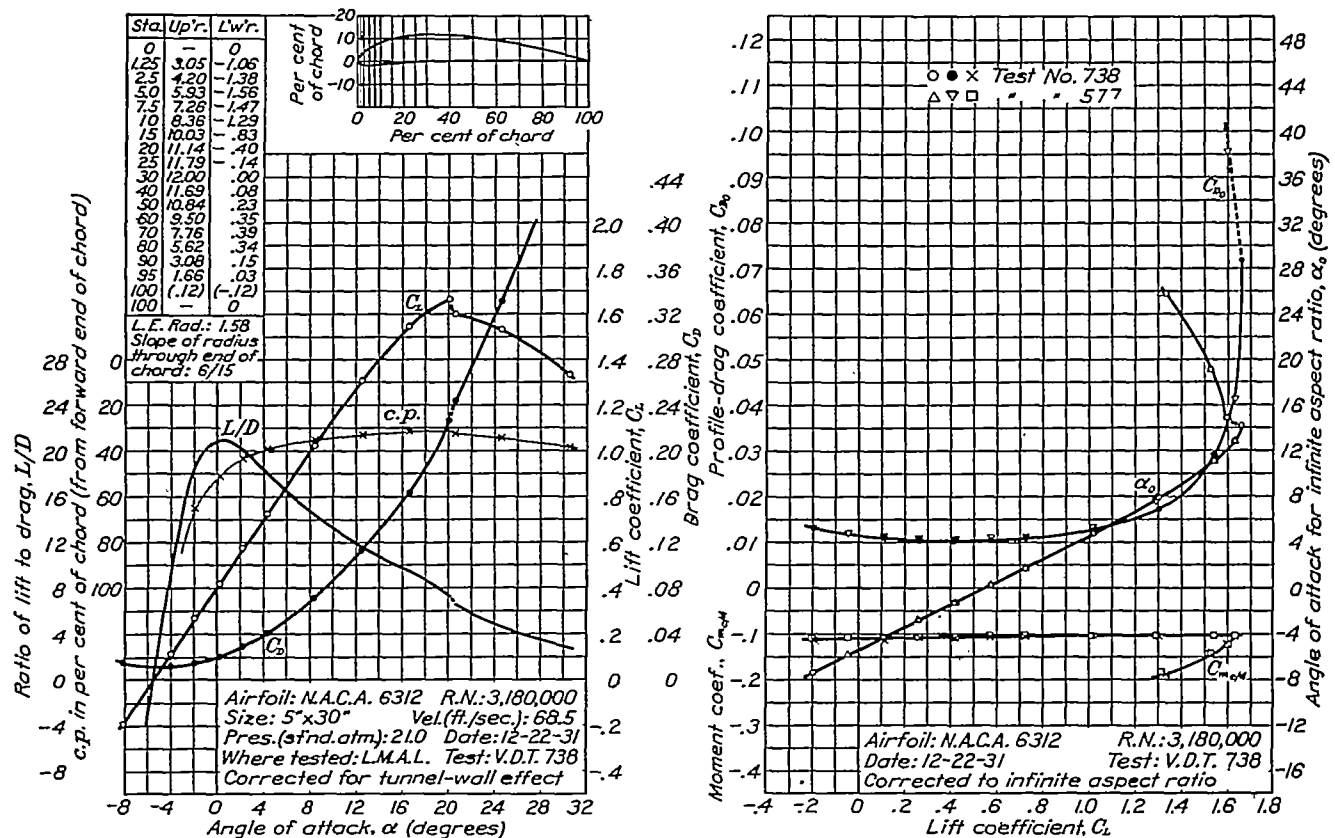
FIGURE 54.—N.A.C.A. 6312 airfoil.
