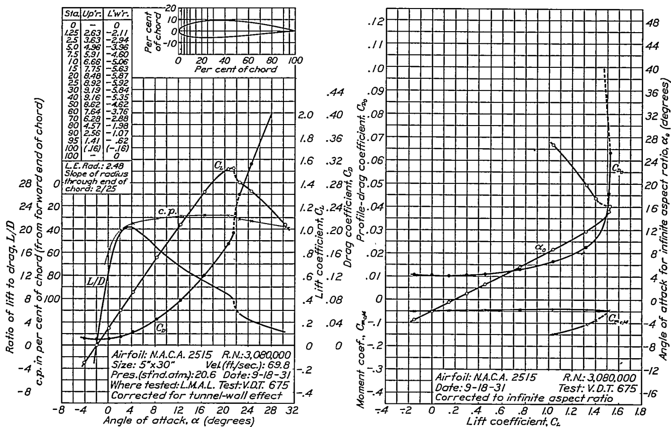
FIGURE 25.—N.A.C.A. 2515 airfoil.
