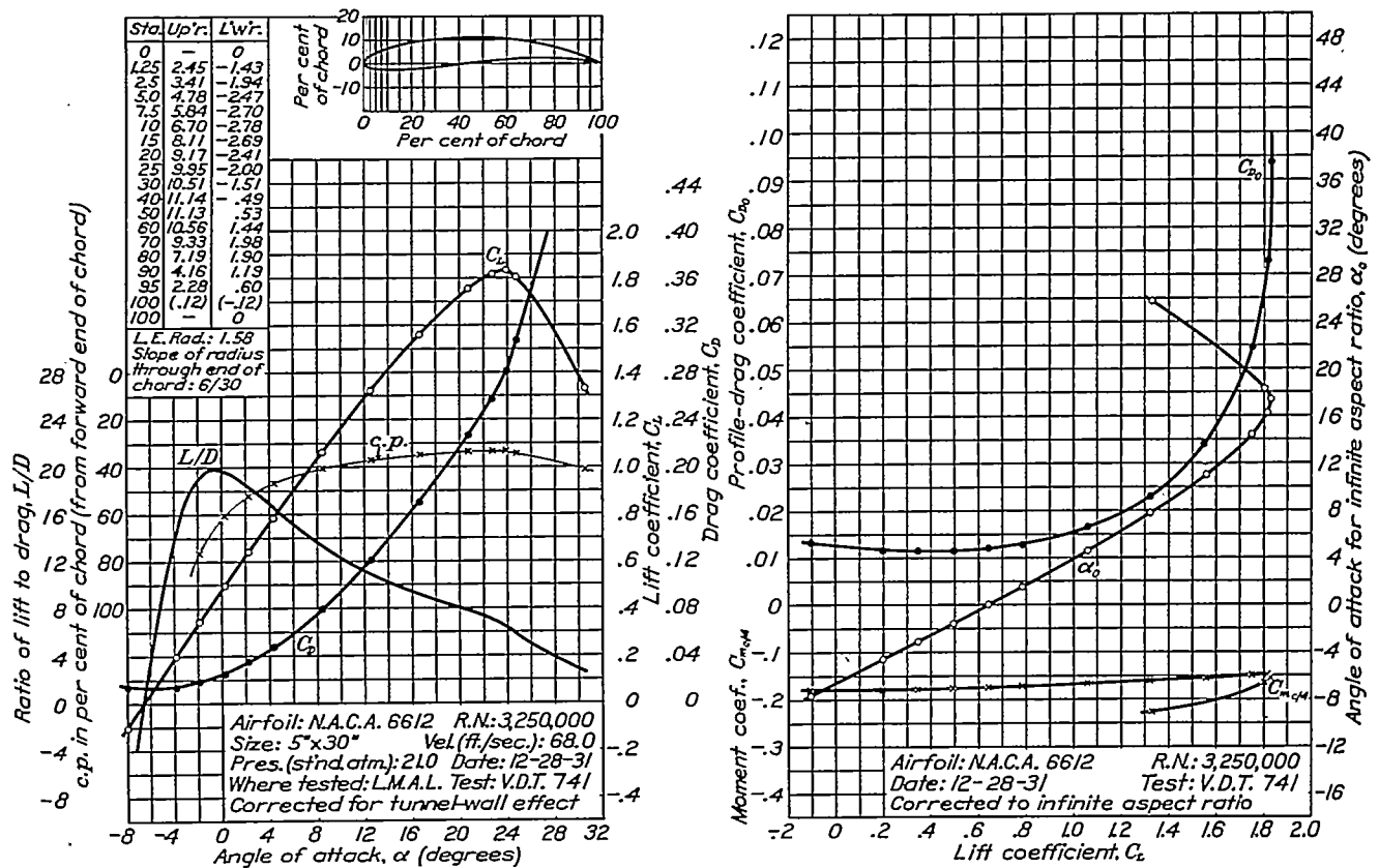
FIGURE 70.—N.A.C.A. 6612 airfoil.
