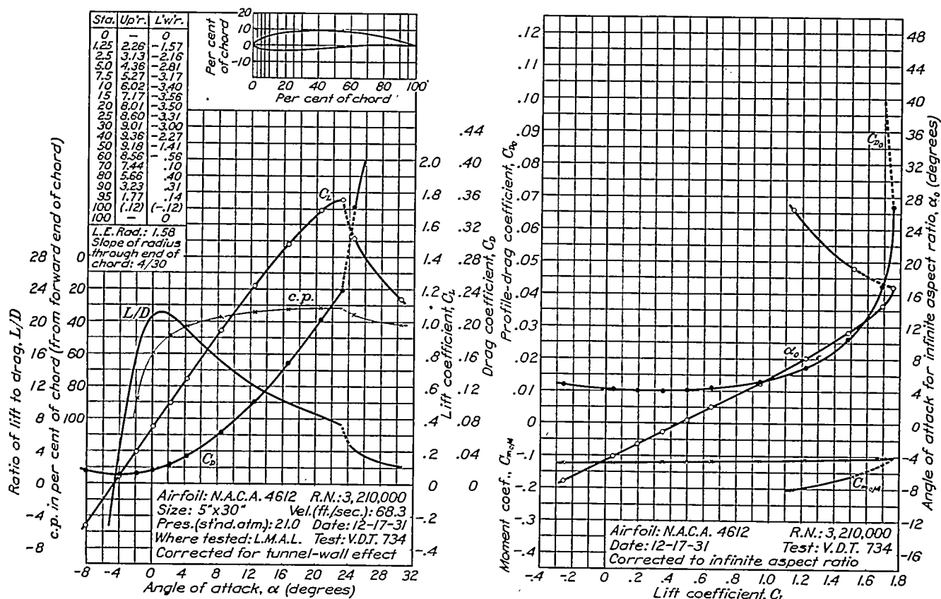
FIGURE 49.—N.A.C.A. 4612 airfoil.
