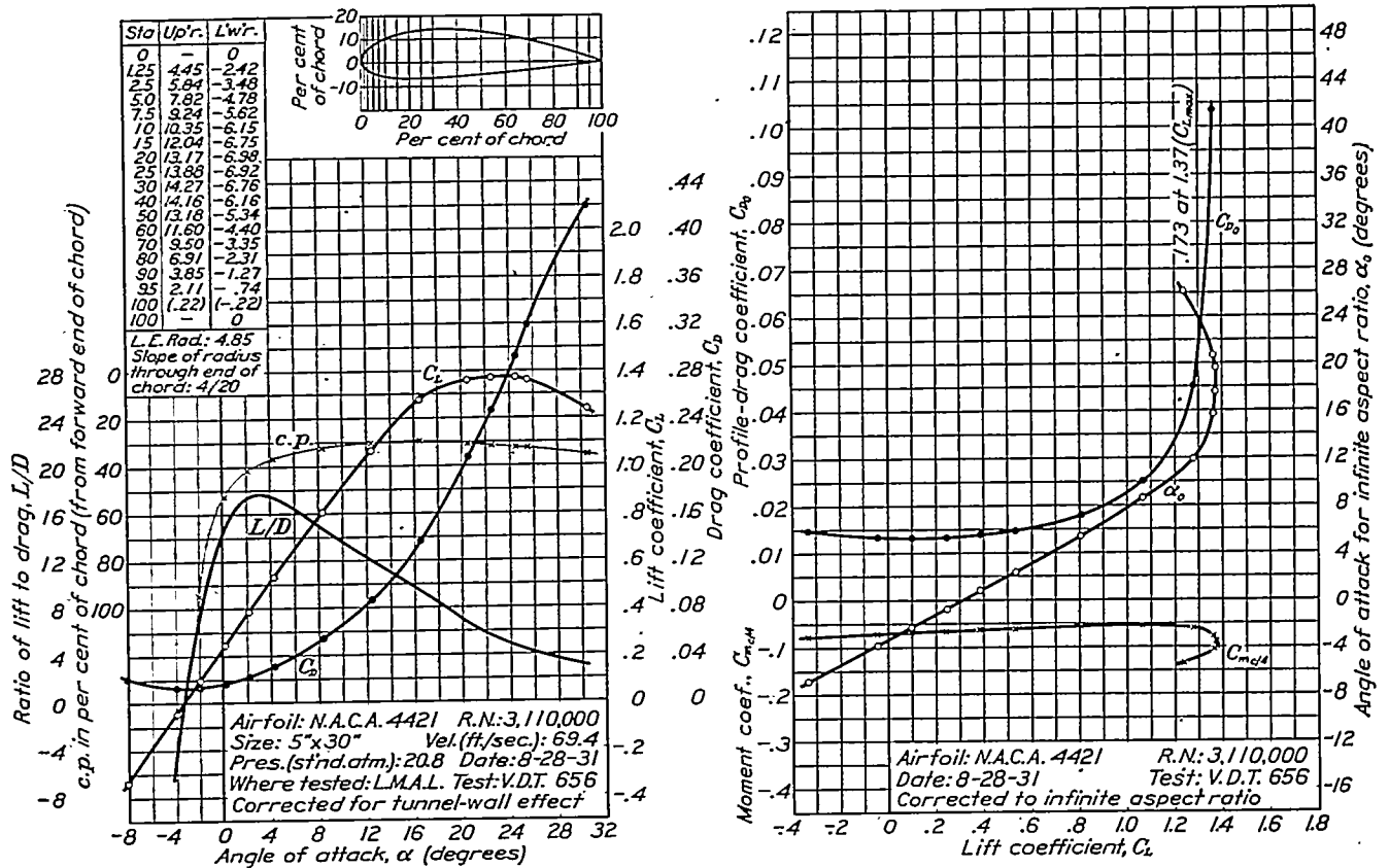
FIGURE 42.—N.A.C.A. 4421 airfoil.
