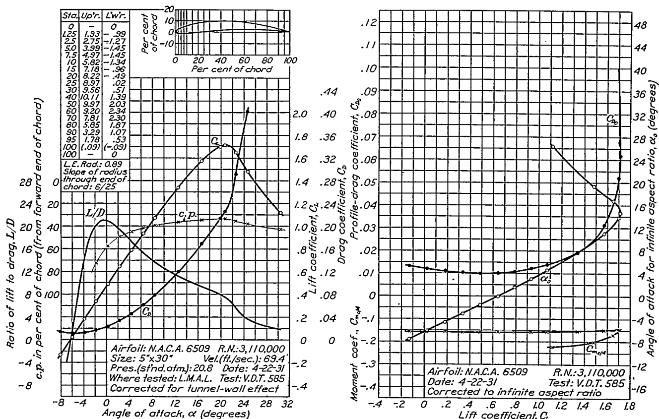
FIGURE 65.—N.A.C.A. 6509 airfoil.
