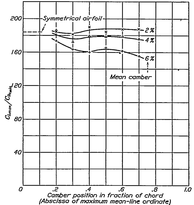
FIGURE 96.—Variation of C_{L_{max}}/C_{D_{p_{min}}} with camber. Results are for 12 percent thick airfoils.
