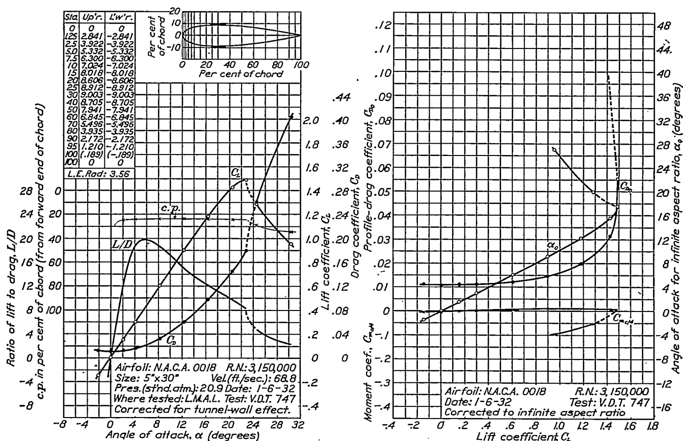
FIGURE 8.—N.A.C.A. 0018 airfoil.
