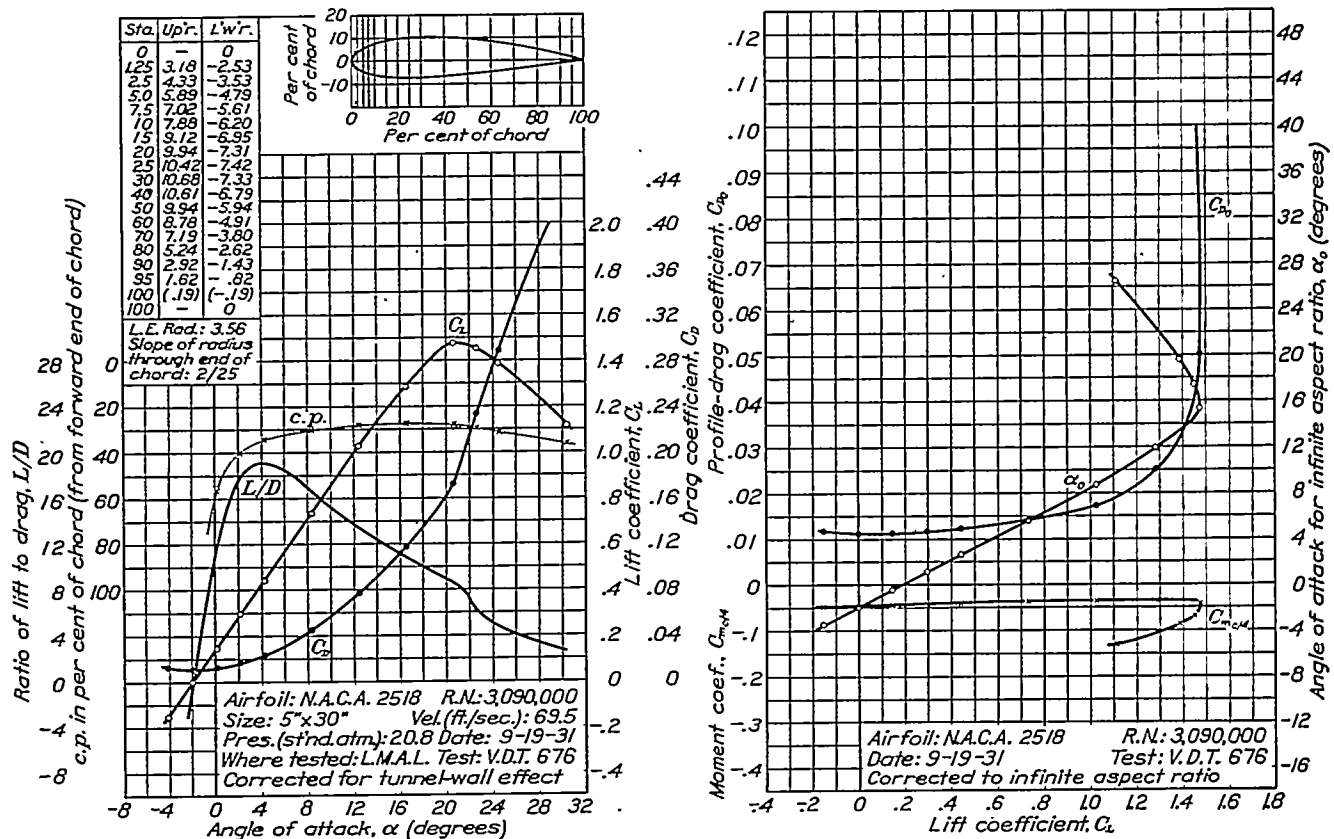
FIGURE 26.—N.A.C.A. 2518 airfoil.
