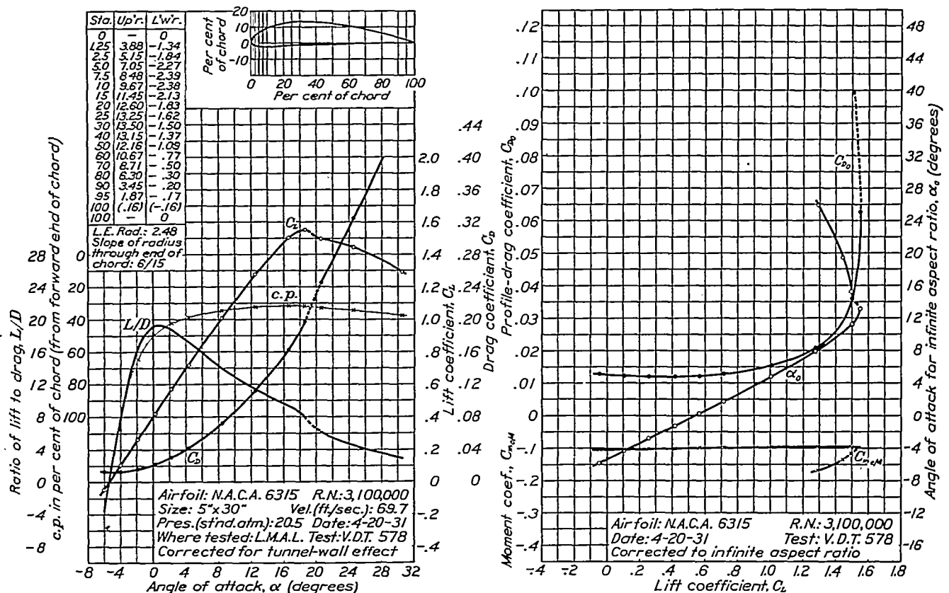
FIGURE 55.—N.A.C.A. 6315 airfoil.
