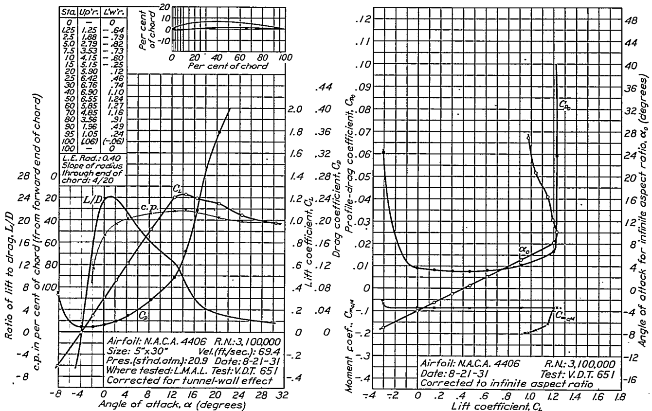
FIGURE 37.—N.A.C.A. 4406 airfoil.
