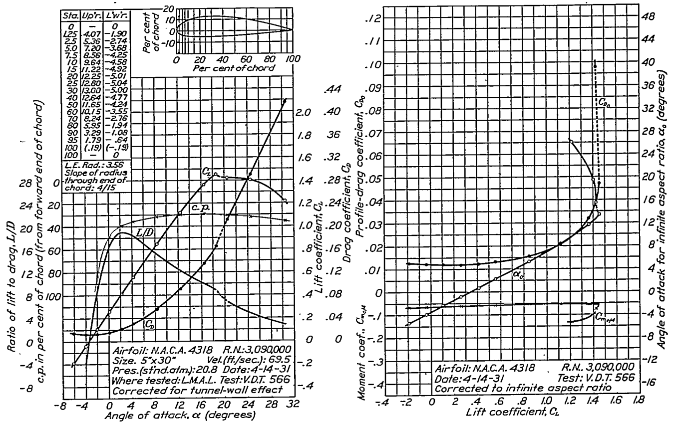
FIGURE 35.—N.A.C.A. 4318 airfoil.
