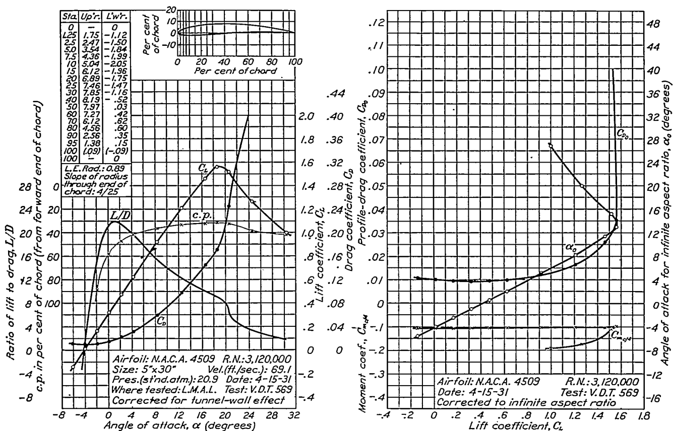
FIGURE 44.—N.A.C.A. 4509 airfoil.
