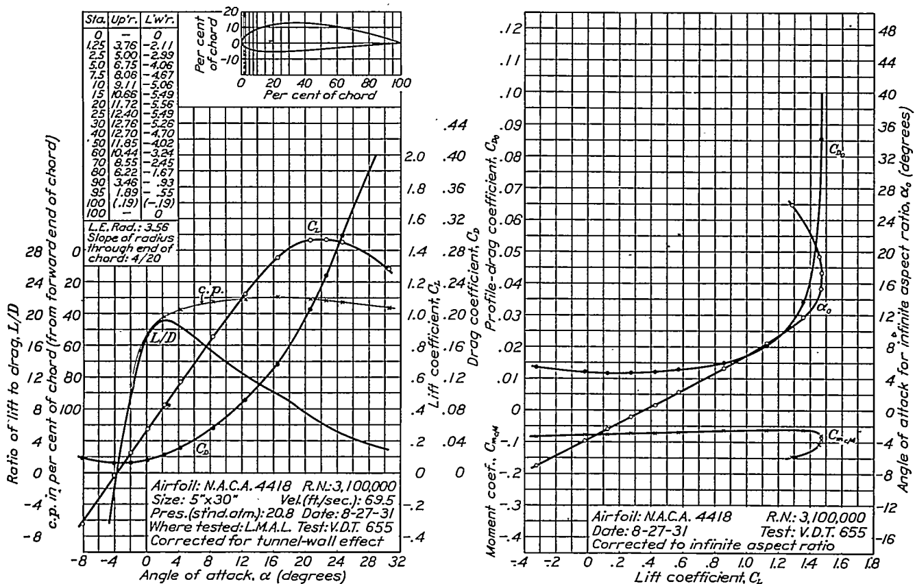
FIGURE 41.—N.A.C.A. 4418 airfoil.
