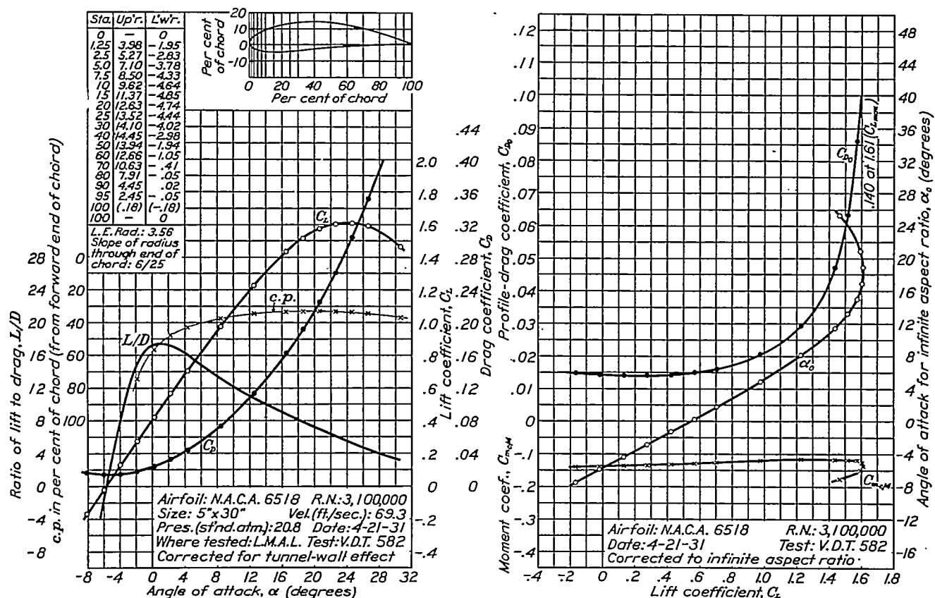
FIGURE 68.—N.A.C.A. 6518 airfoil.
