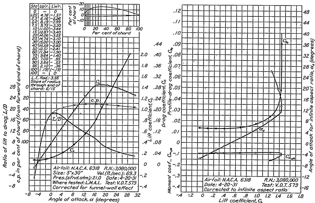
FIGURE 56.—N.A.A. 6318 airfoil.
