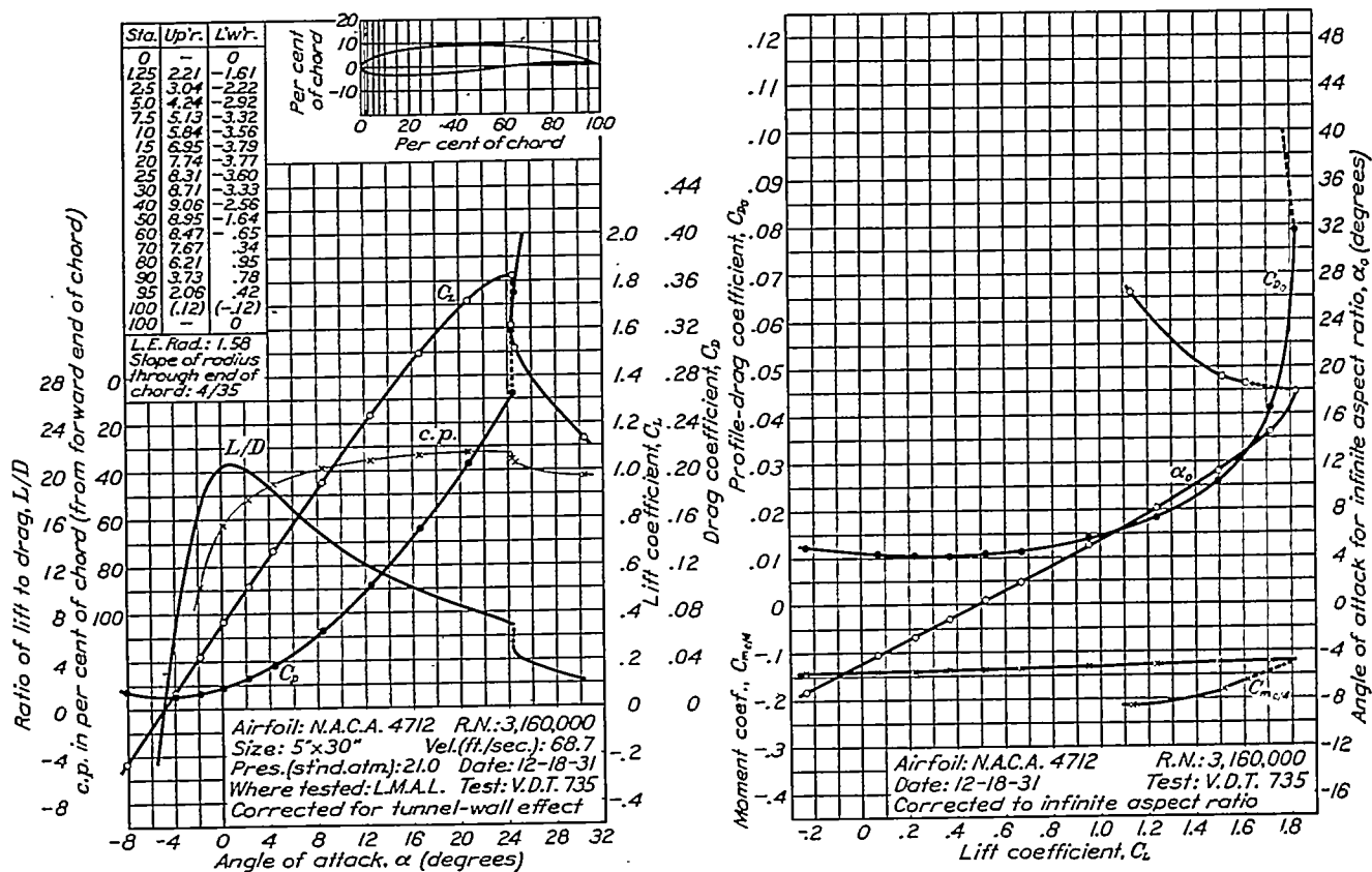
FIGURE 50.—N.A.C.A. 4712 airfoil.
