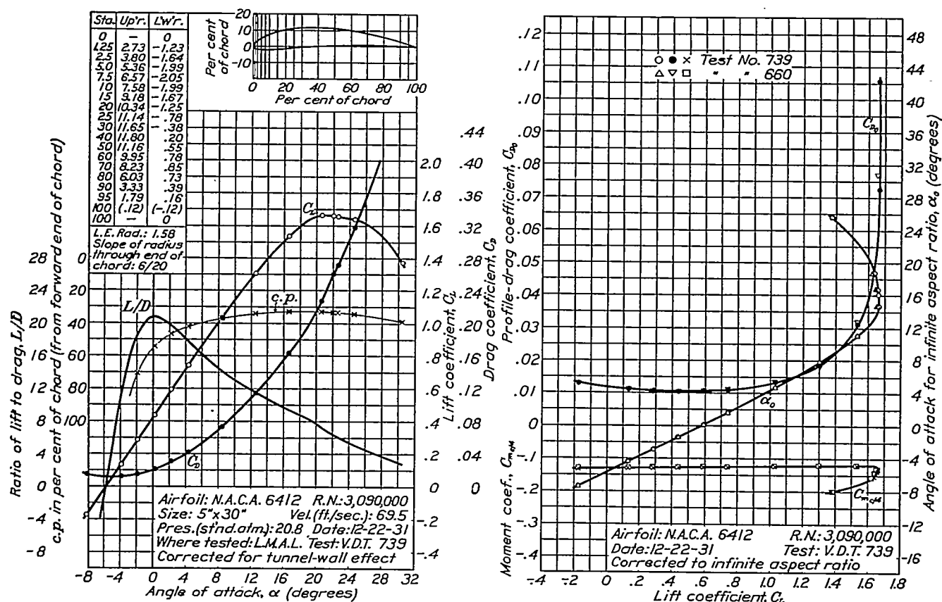
FIGURE 60.—N.A.C.A. 6412 airfoil.
