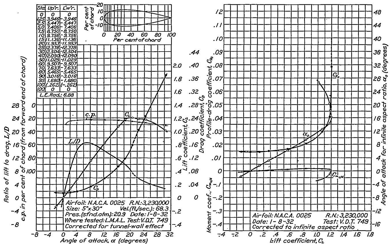
FIGURE 10.—N.A.C.A. 0025 airfoil.
