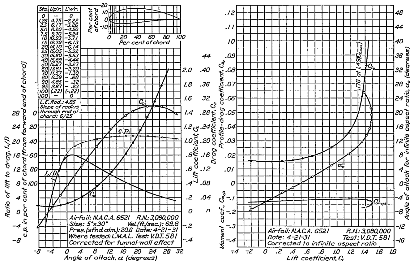
FIGURE 69.—N.A.C.A. 6521 airfoil.
