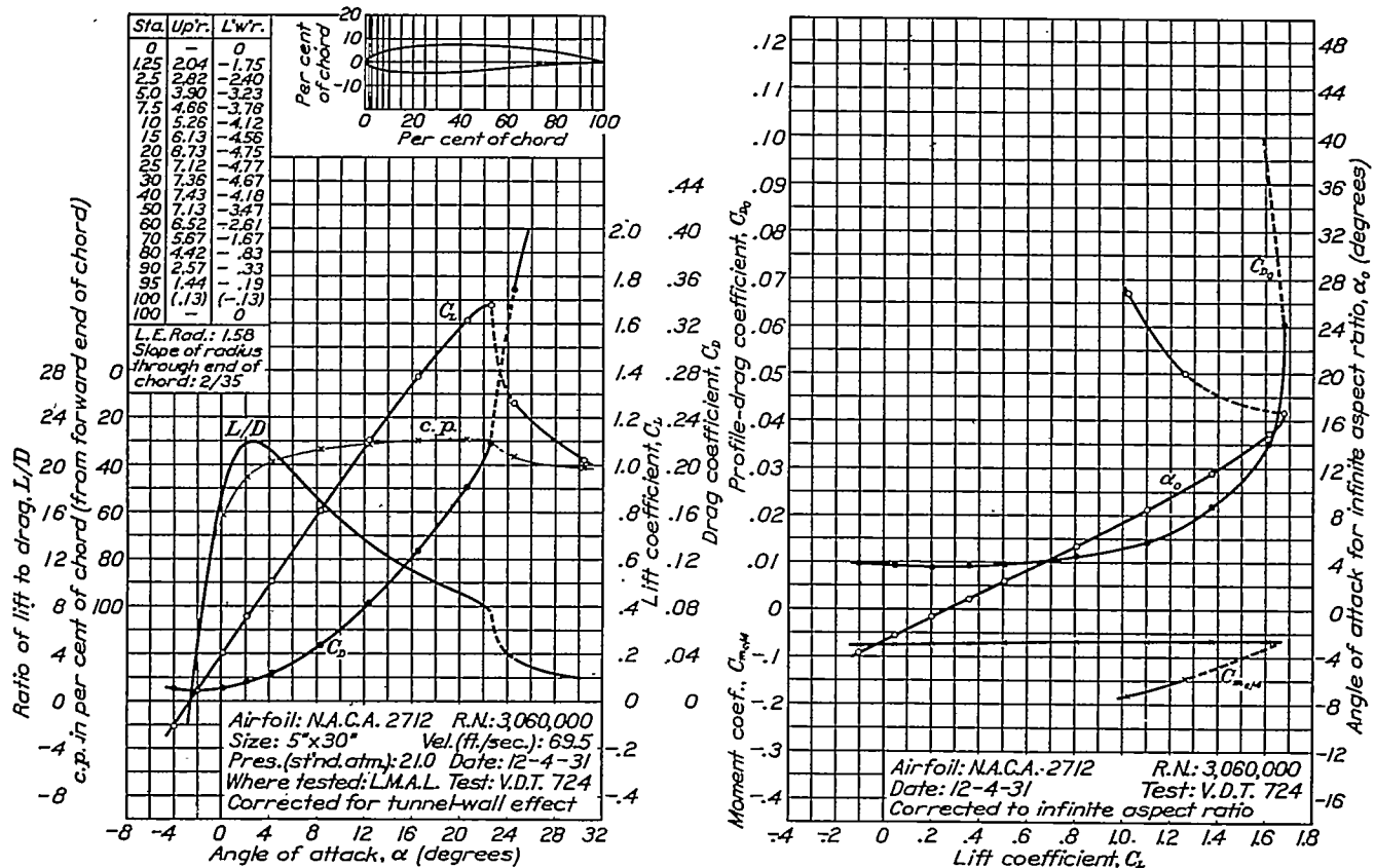
FIGURE 29.—N.A.C.A. 2712 airfoil.
