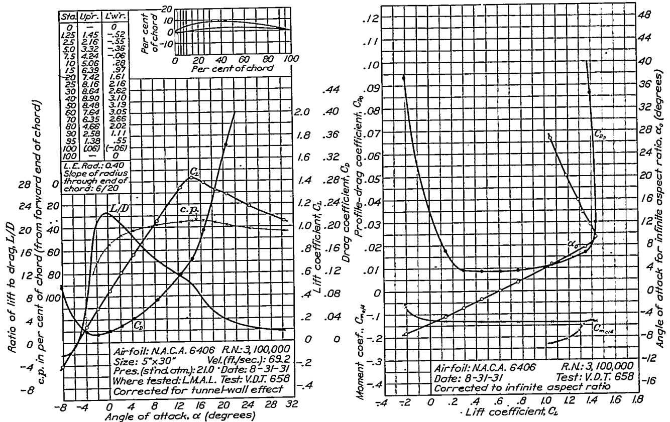
FIGURE 58.—N.A.C.A. 6406 airfoil.
