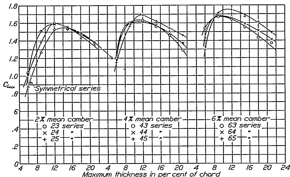
FIGURE 85.—Variation of maximum lift with thickness.
