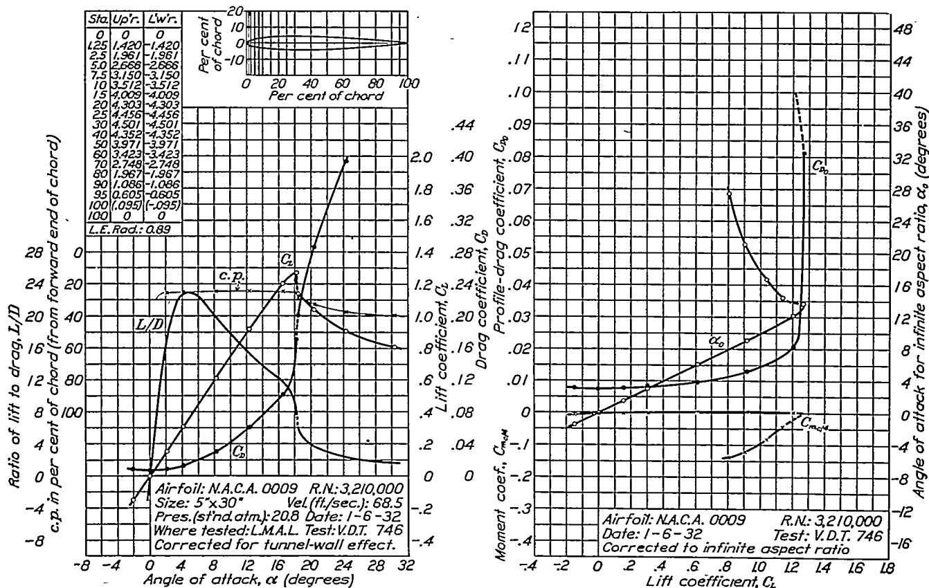
FIGURE 5.—N.A.C.A. 0009 airfoil.
