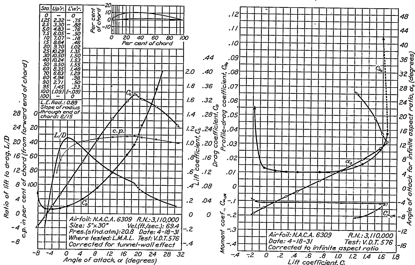
FIGURE 53.—N.A.C.A. 6309 airfoil.
