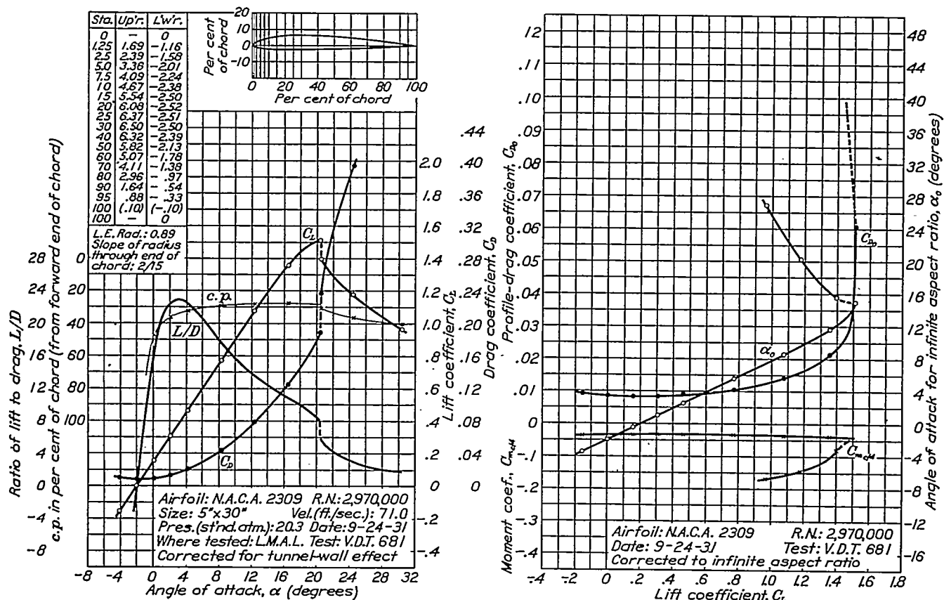
FIGURE 13.—N.A.C.A. 2309 airfoil.
