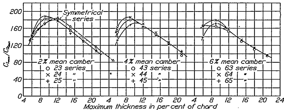
FIGURE 95.—Variation of C_{L_{max}}/C_{D_{p_{min}}} with thickness.
