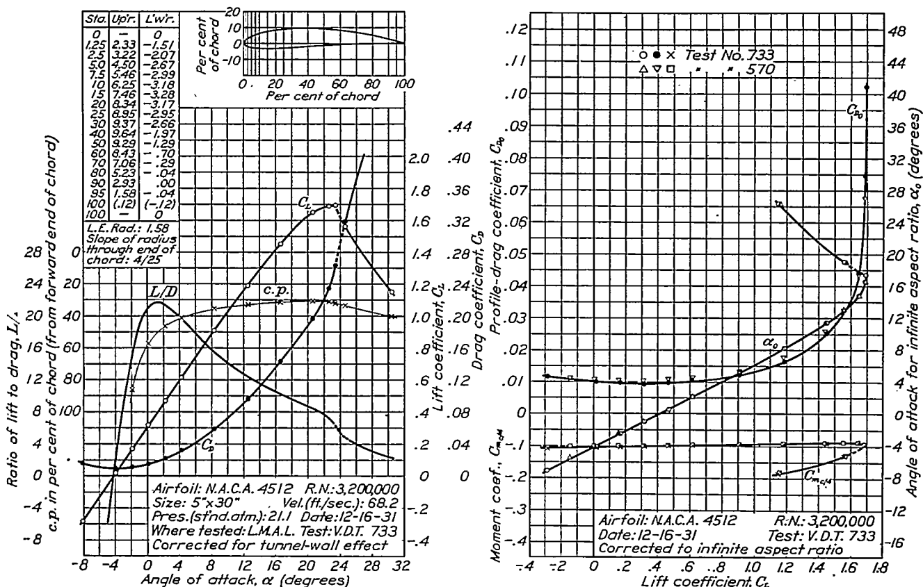
FIGURE 45.—N.A.C.A. 4512 airfoil.
