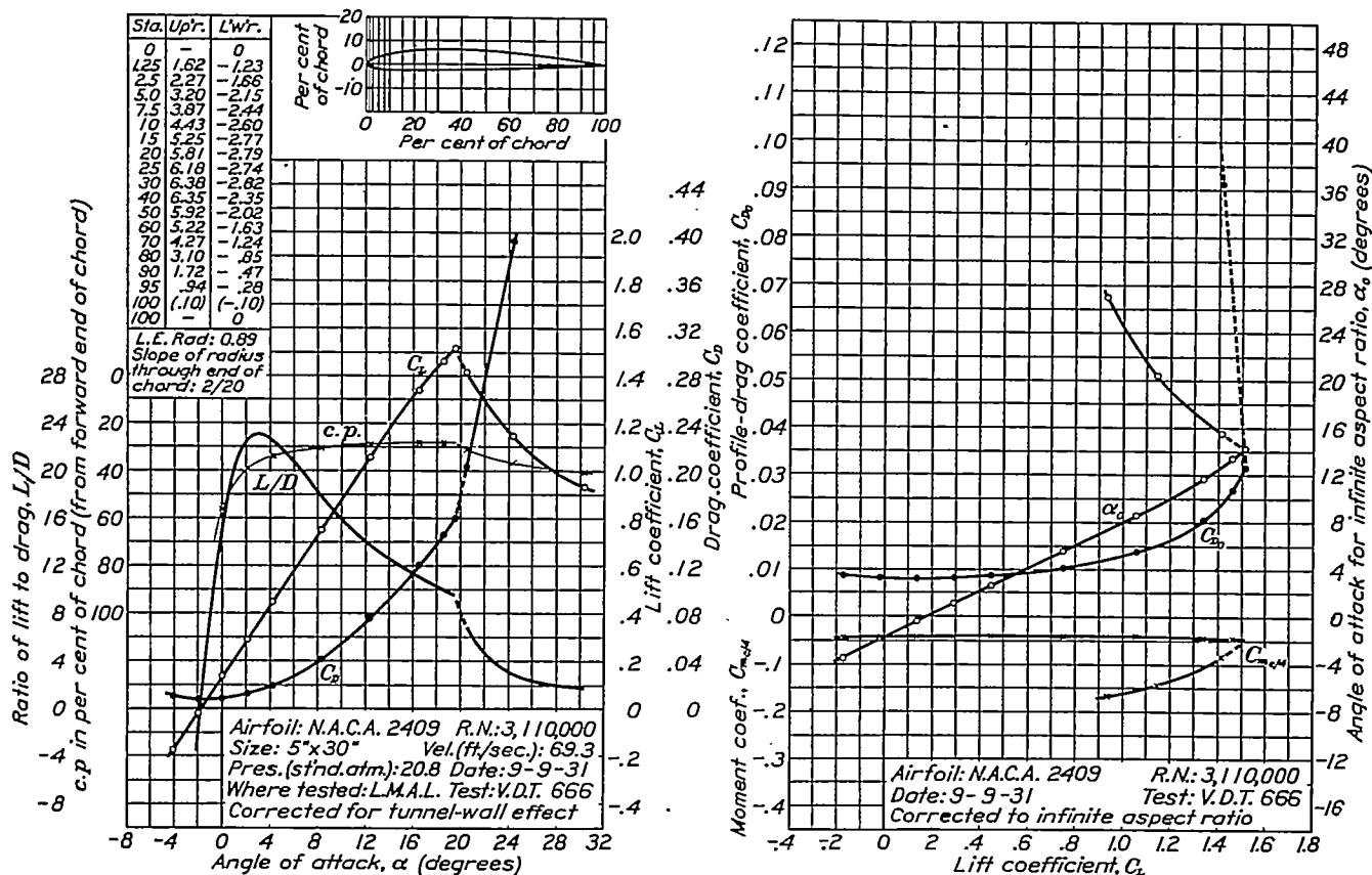
FIGURE 17.—N.A.C.A. 2409 airfoil.
