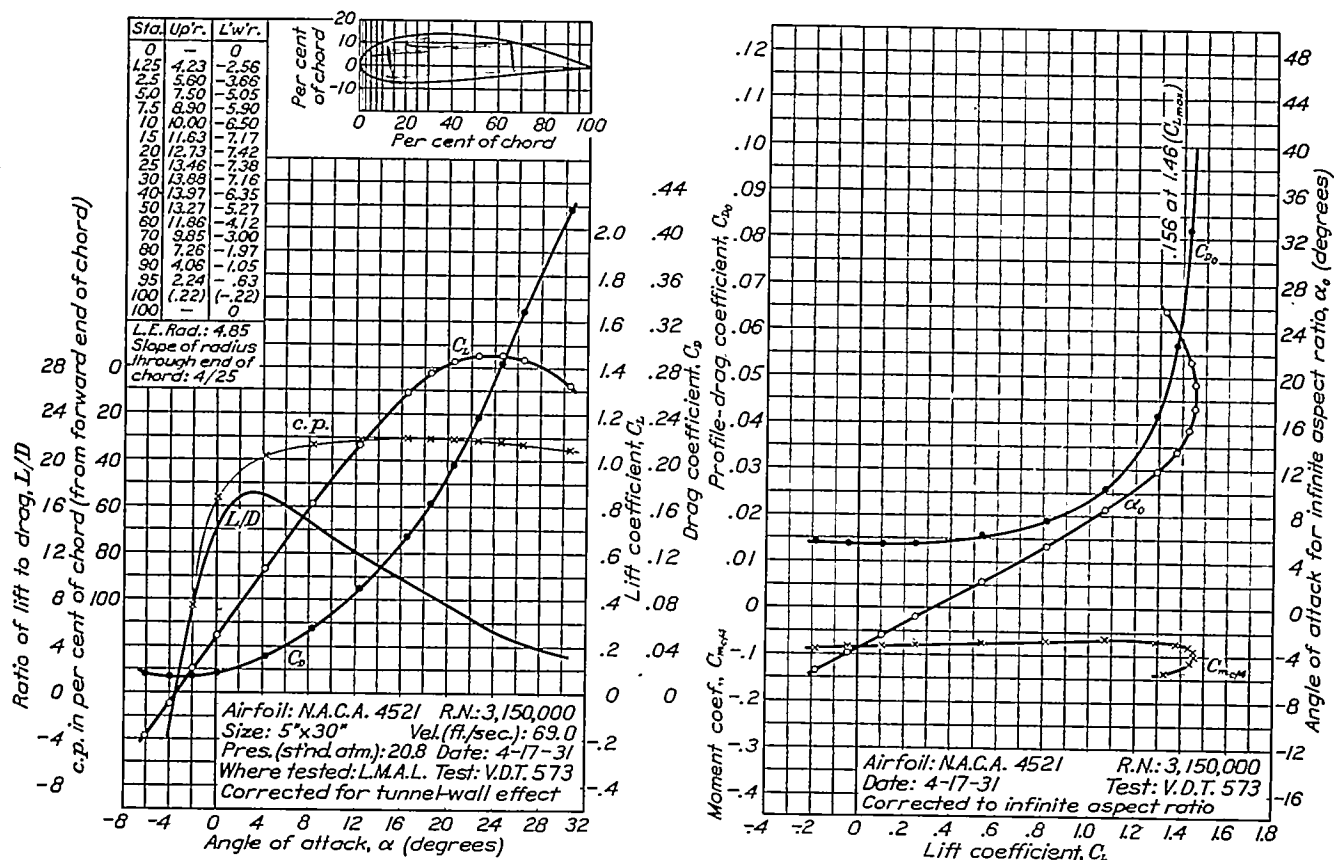
FIGURE 48.—N.A.C.A. 4521 airfoil.
