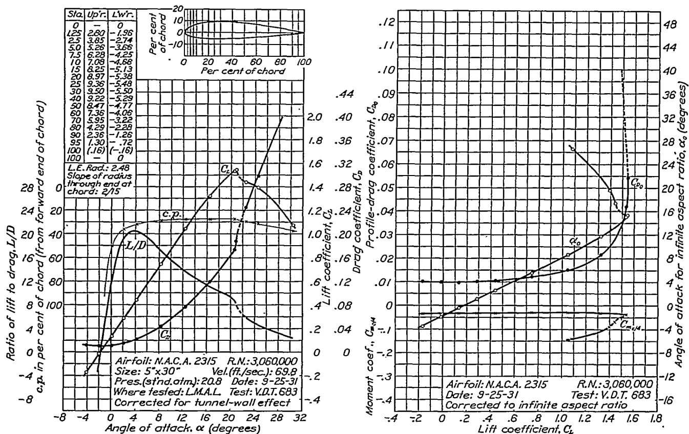
FIGURE 15.—N.A.C.A. 2315 airfoil.
