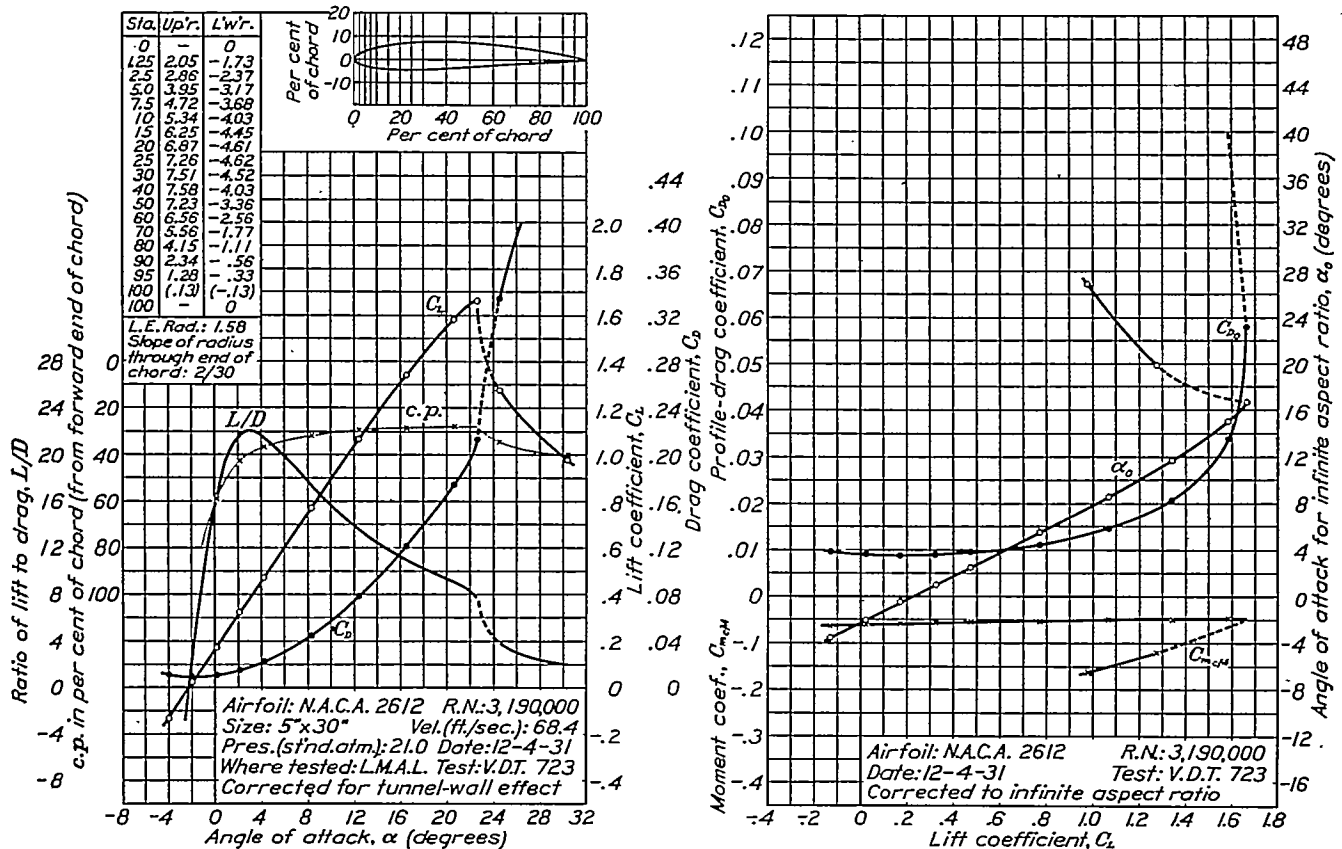
FIGURE 28.—N.A.C.A. 2612 airfoil.
