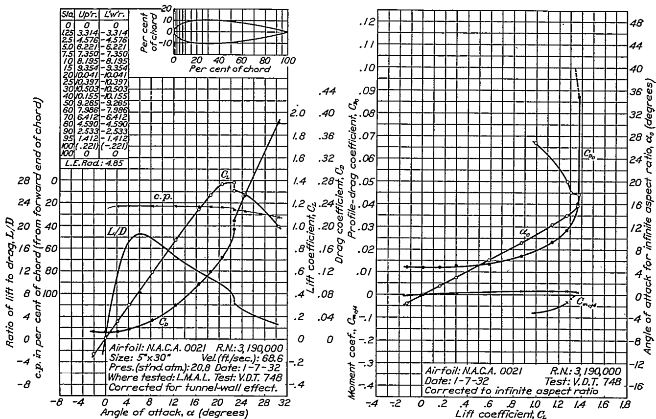
FIGURE 9.—N.A.C.A. 0021 airfoil.
