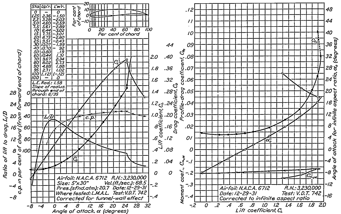
FIGURE 71.—N.A.C.A. 6712 airfoil.
