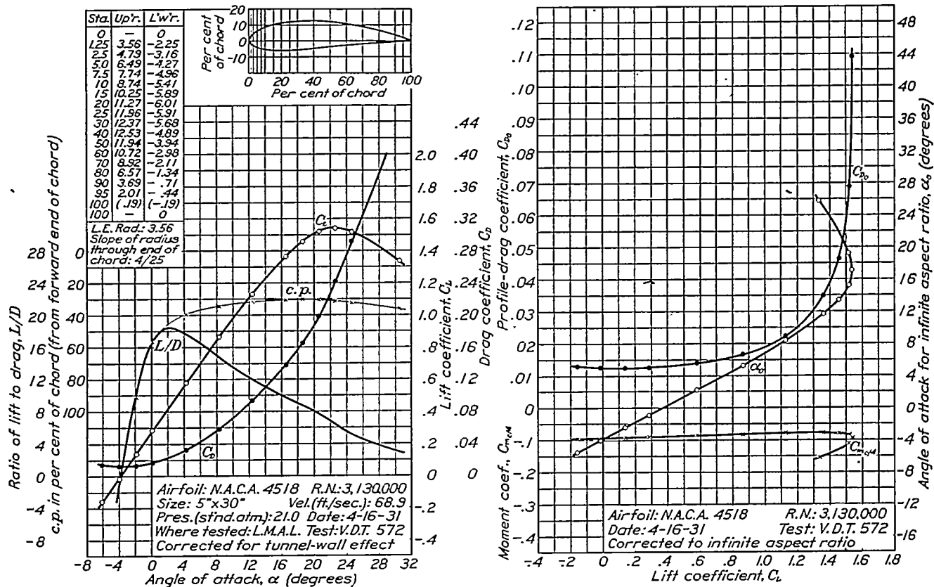
FIGURE 47.—N.A.C.A. 4518 airfoil.
