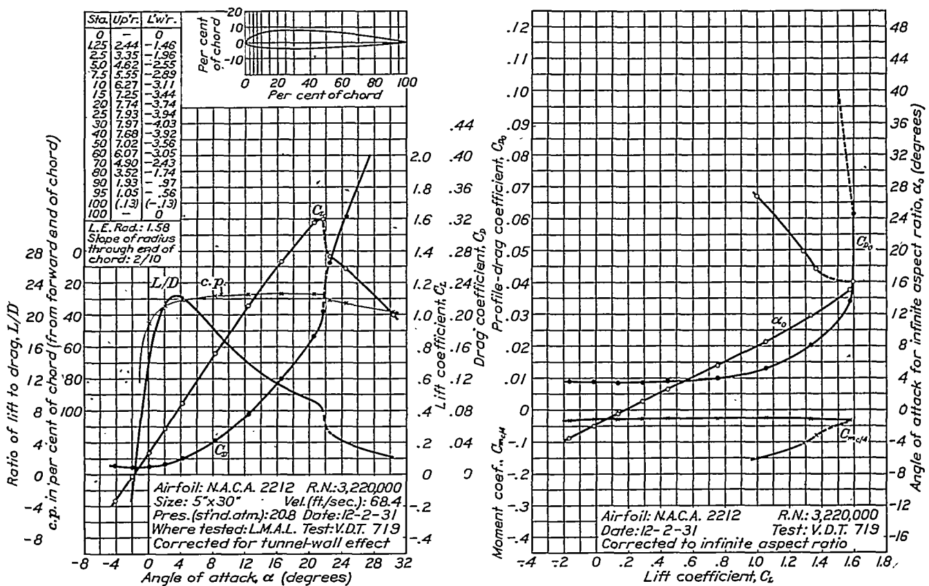
FIGURE 11.—N.A.C.A. 2212 airfoil.
