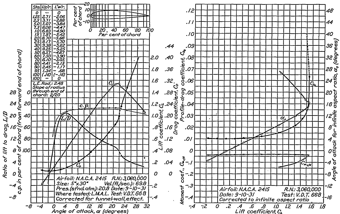
FIGURE 19.—N.A.C.A. 2415 airfoil.
