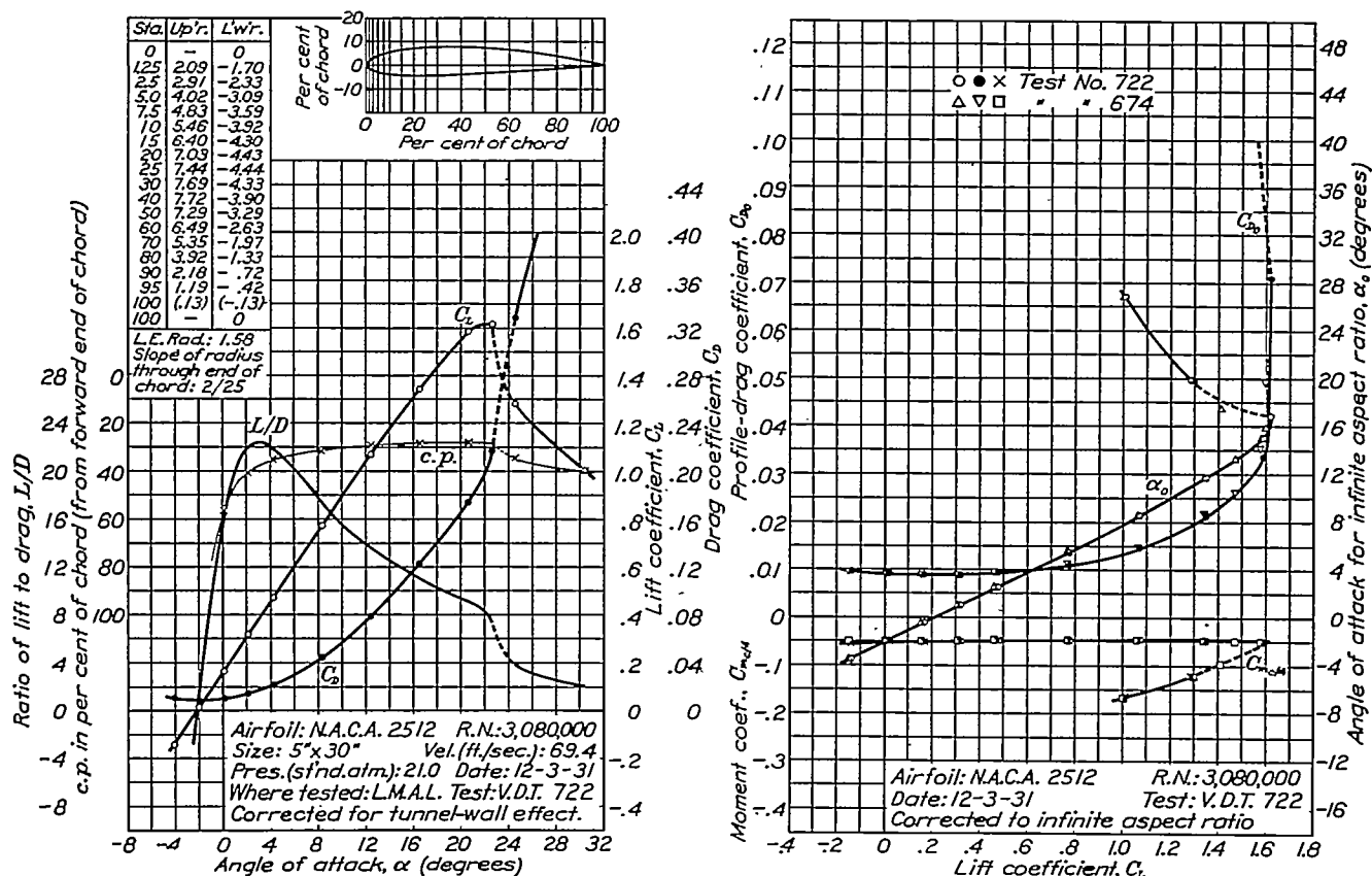
FIGURE 24.—N.A.C.A. 2512 airfoil.
