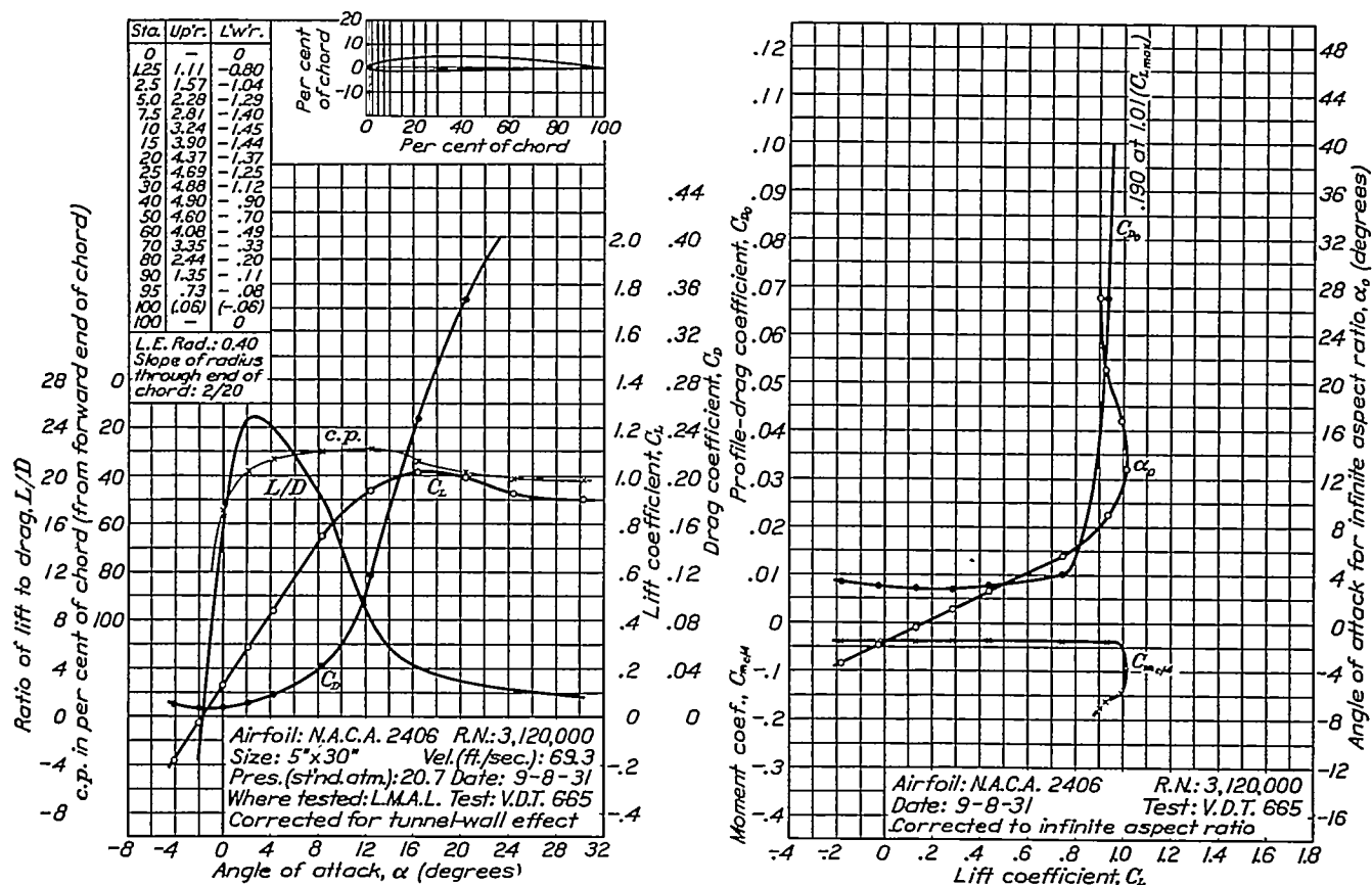
FIGURE 16.—N.A.C.A. 2406 airfoil.
