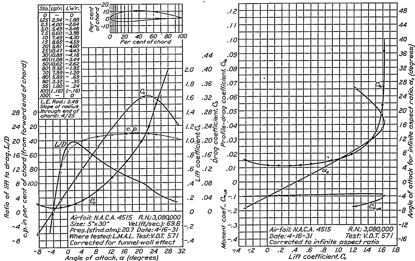
FIGURE 46.—N.A.C.A. 4515 airfoil.
