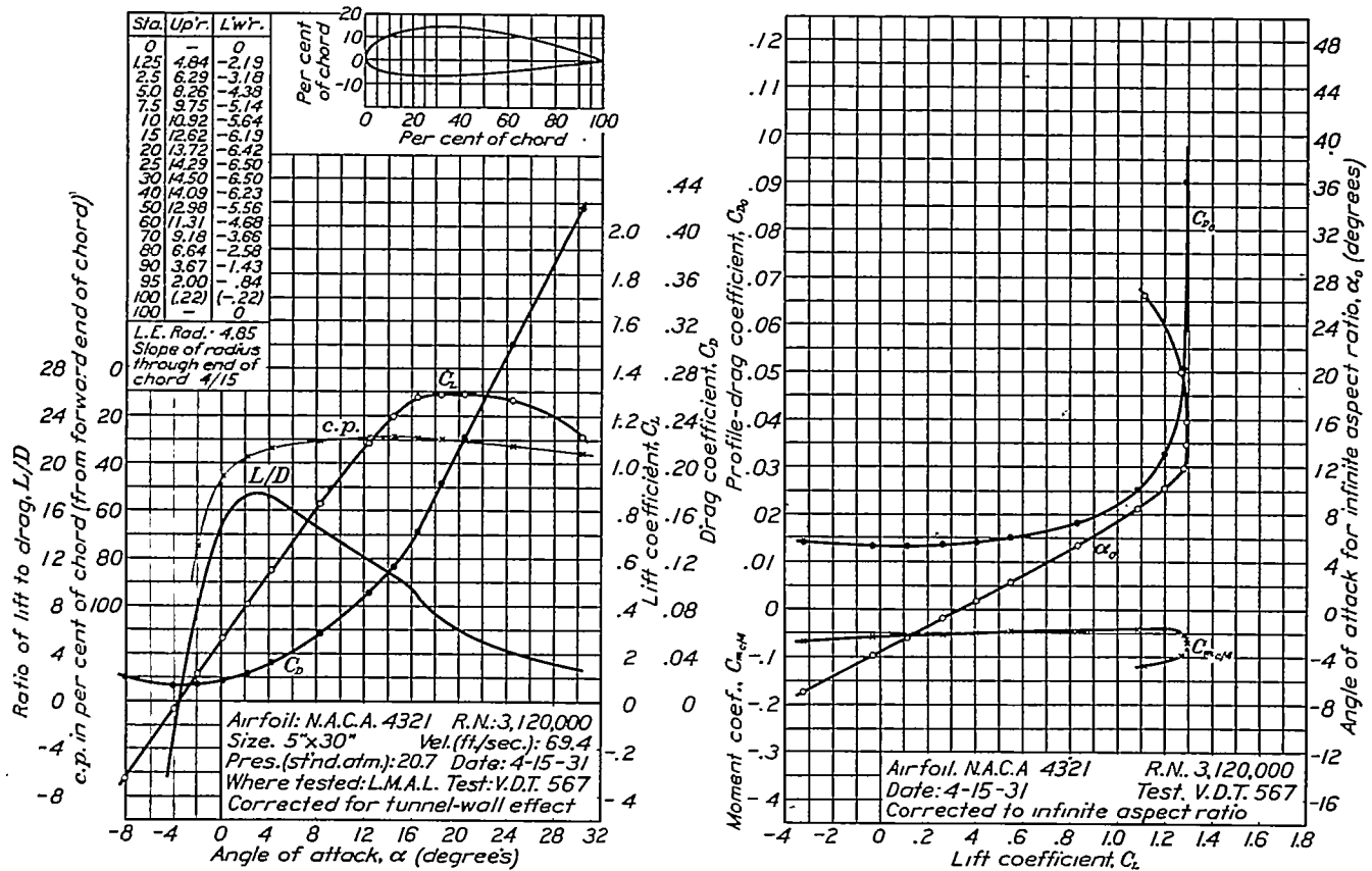
FIGURE 36.—N.A.C.A. 4321 airfoil.
