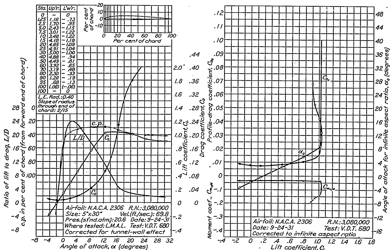
FIGURE 12.—N.A.C.A. 2306 airfoil.
