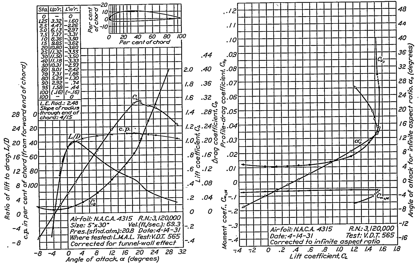
FIGURE 34.—N.A.C.A. 4315 airfoil.
