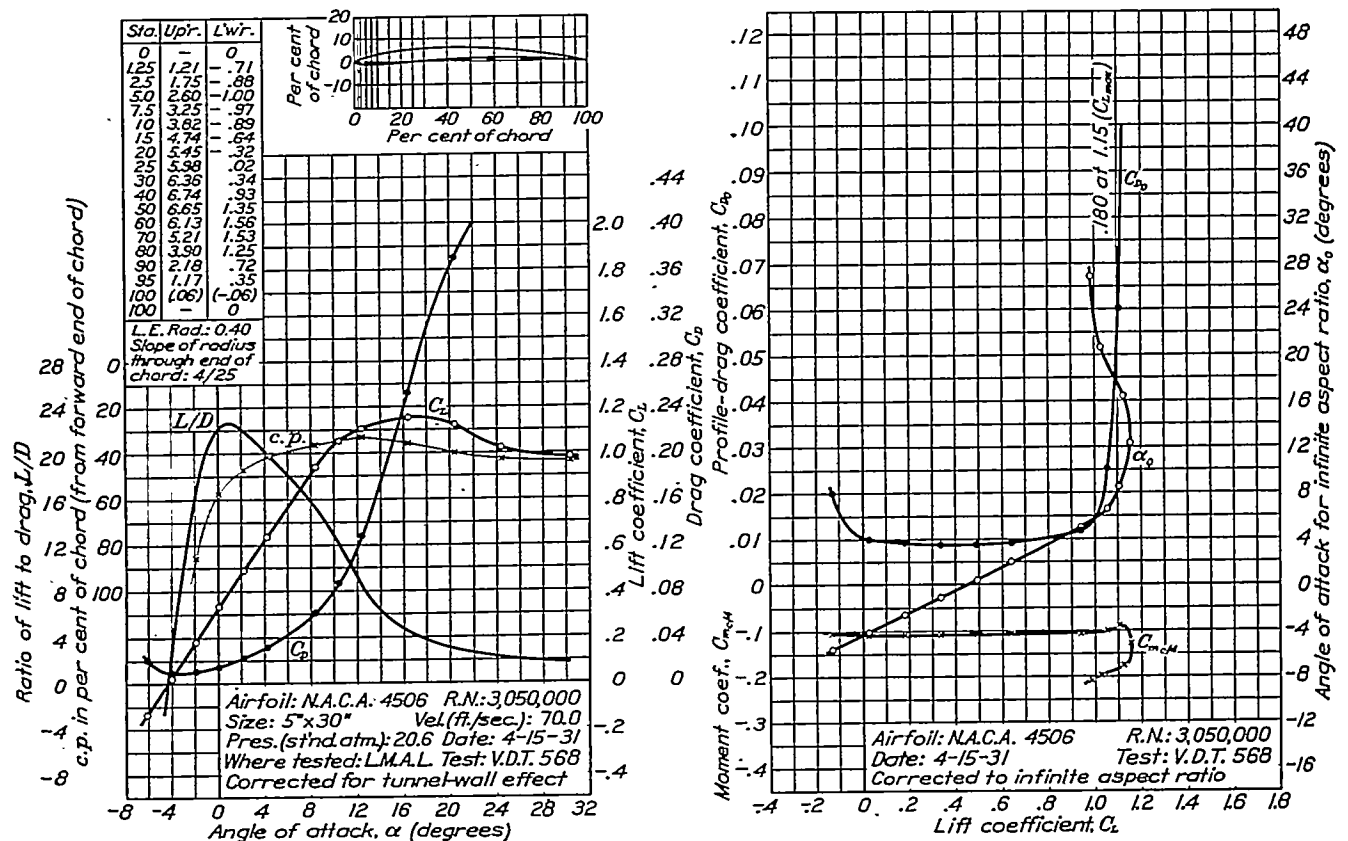
FIGURE 43.—N.A.C.A. 4506 airfoil.
