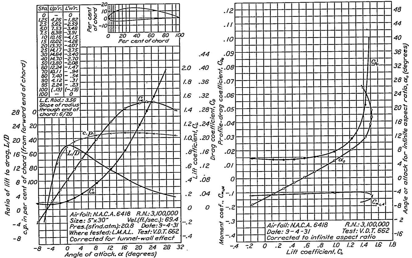
FIGURE 62.—N.A.C.A. 6418 airfoil.
