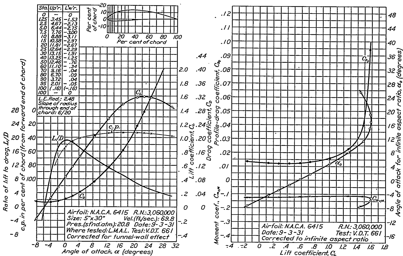
FIGURE 61.—N.A.C.A. 6415 airfoil.
