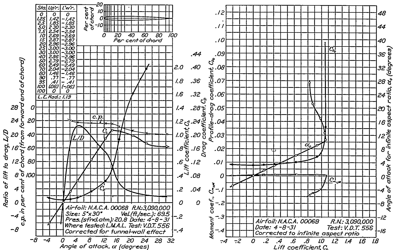
FIGURE 73.—N.A.C.A. 0006B airfoil.
