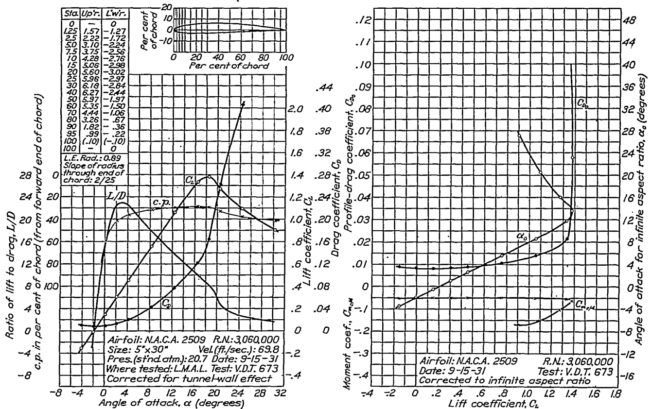
FIGURE 23.—N.A.C.A. 2509 airfoil.
