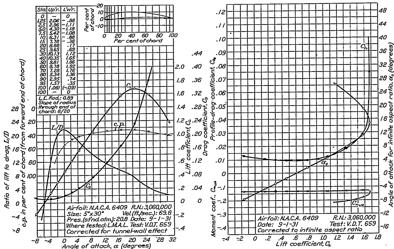
FIGURE 59.—N.A.C.A. 6409 airfoil.
