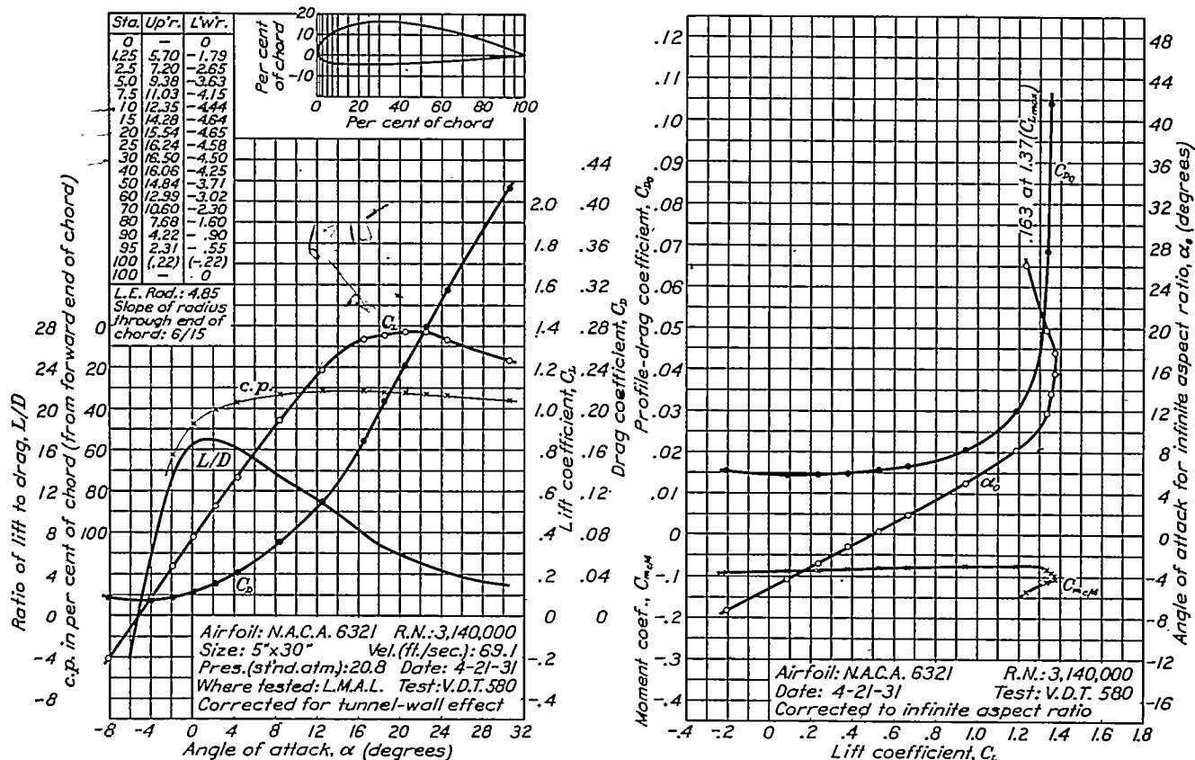
FIGURE 57.—N.A.A. 6321 airfoil.
