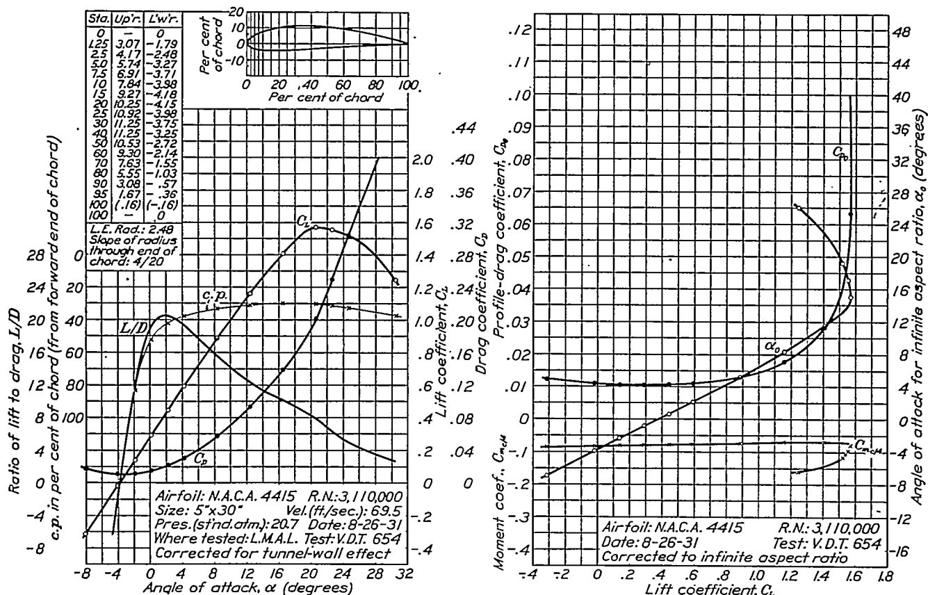
FIGURE 40.—N.A.C.A. 4415 airfoil.
