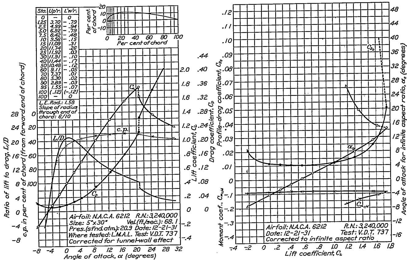
FIGURE 51.—N.A.C.A. 6212 airfoil.
